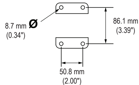
Mounting Bracket
