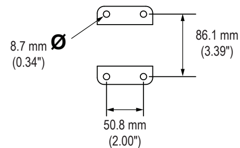
Mounting Bracket
