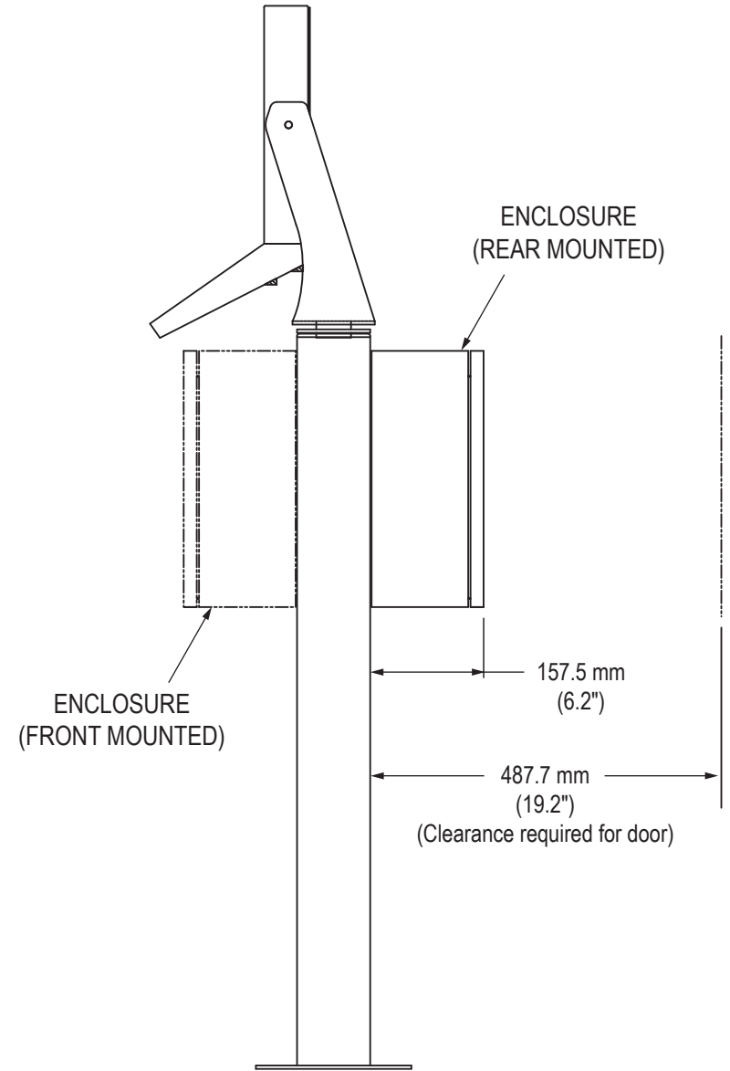
Side View
