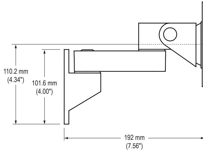
Side View with 3.5" Extension Arm
